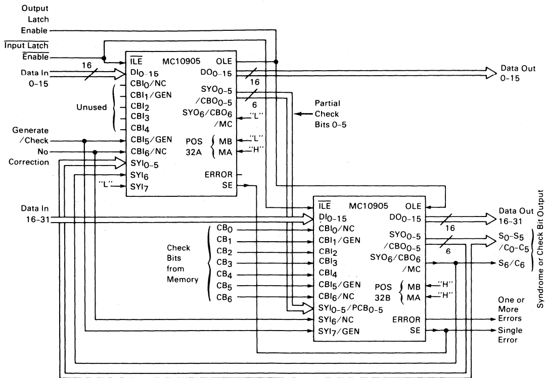
FIGURE 4 — 32-BIT DATA CONFIGURATION
