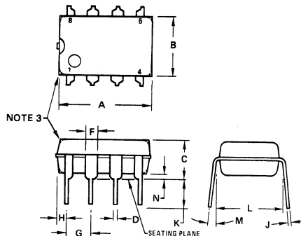
P SUFFIX PLASTIC PACKAGE CASE 626-04
