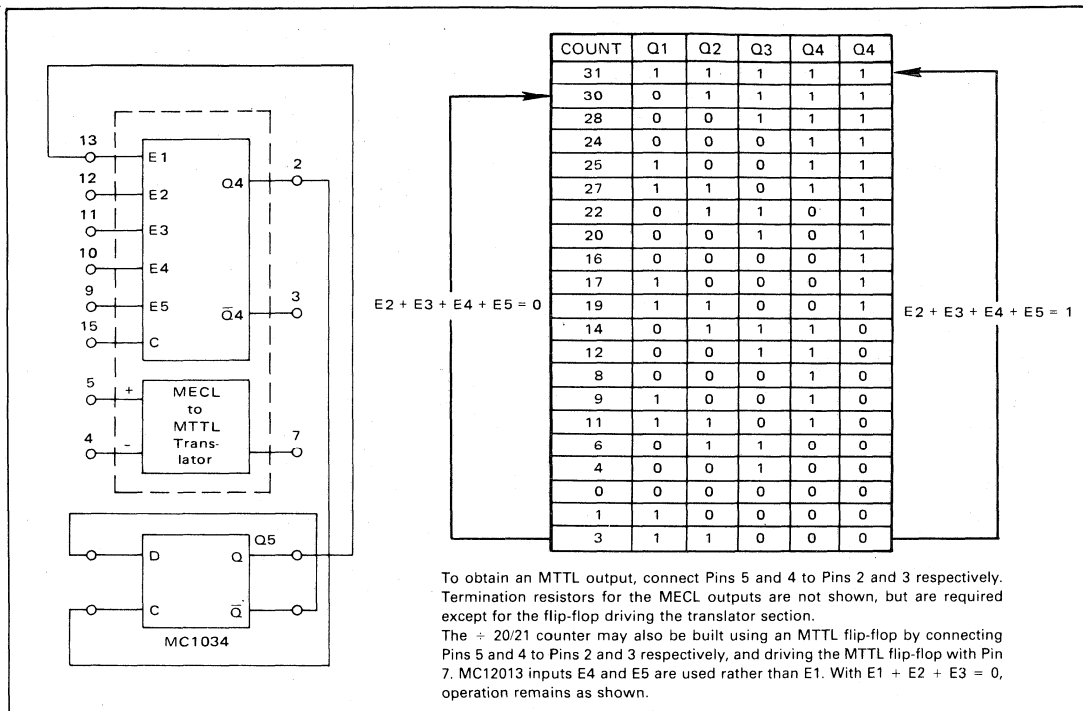
FIGURE 10 – DIVIDE BY 40/41 (MC12013/MC12513)
