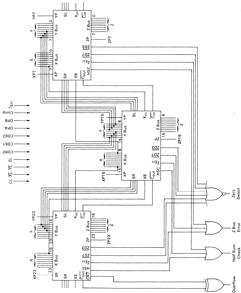
FIGURE 3 — 24-BIT ALU
