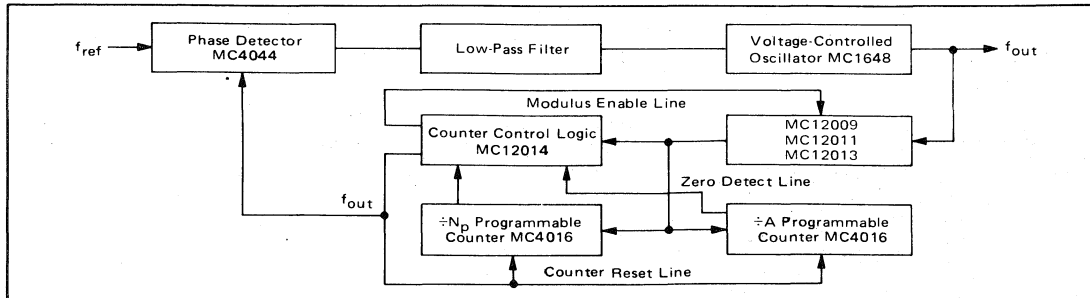
FIGURE 2 – TYPICAL FREQUENCY SYNTHESIZER APPLICATION
