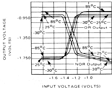
FIGURE 6 — TYPICAL TRANSFER CHARACTERISTICS AS A FUNCTION OF TEMPERATURE (MECL 10K)
