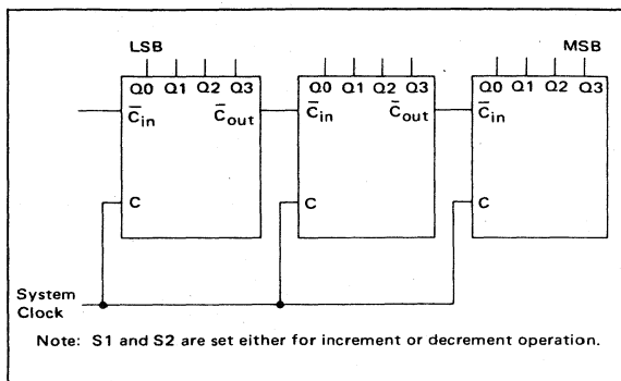
FIGURE 1 — 12 BIT SYNCHRONOUS COUNTER
