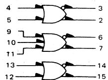
Triple 2-3-2 Input OR/NOR Gate
