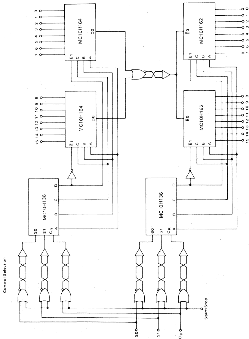
FIGURE 1 — HIGH SPEED 16-BIT MULTIPLEXER/DEMULTIPLEXER
