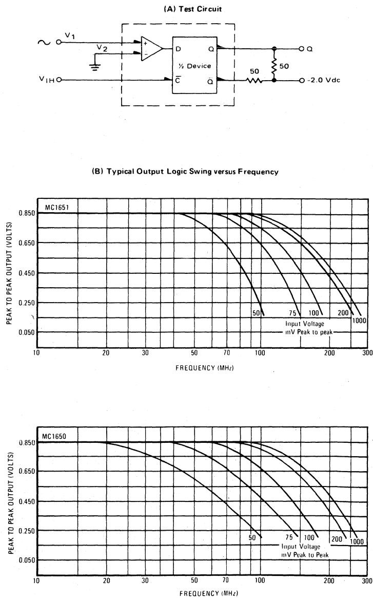
FIGURE 7 – OUTPUT VOLTAGE SWING versus FREQUENCY
