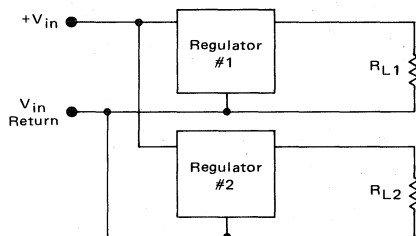
FIGURE 27 — REGULATOR GROUND CONNECTION
