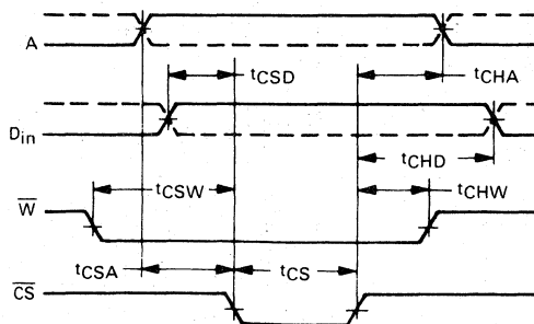
FIGURE 1 — CHIP ENABLE STROBE MODE
