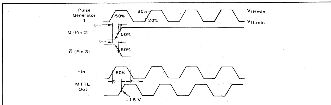
FIGURE 3 – AC VOLTAGE WAVEFORMS
