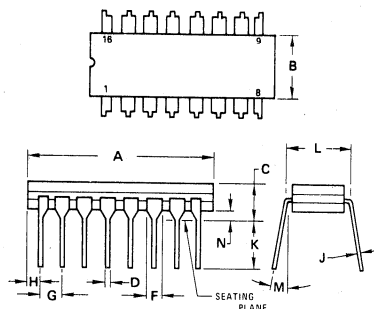
L SUFFIX CERAMIC PACKAGE CASE 620-02
