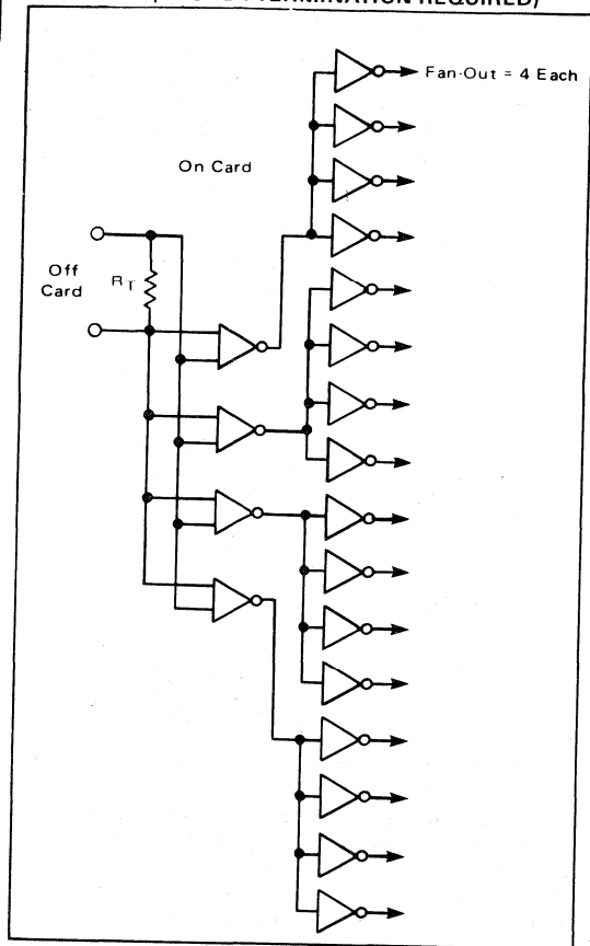
FIGURE 27 — 64 FANOUT CLOCK DISTRIBUTION (PROPER TERMINATION REQUIRED)
