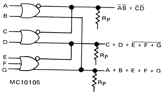
FIGURE 28 — USE OF WIRE-OR AND COMPLEMENTARY OUTPUTS
