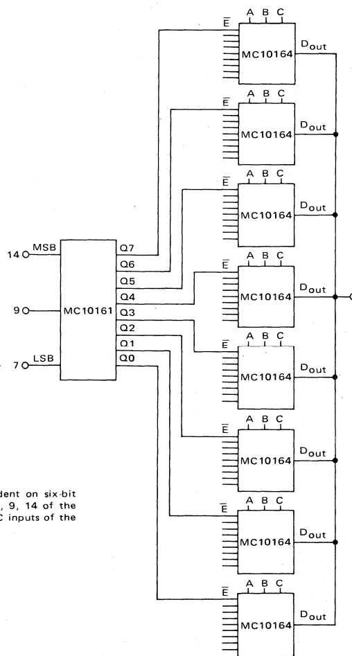
FIGURE 1 - 1-OF-64 LINE MULTIPLEXER
