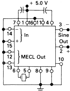
FIGURE 2 — SINE WAVE OUTPUT + 5.0 V
