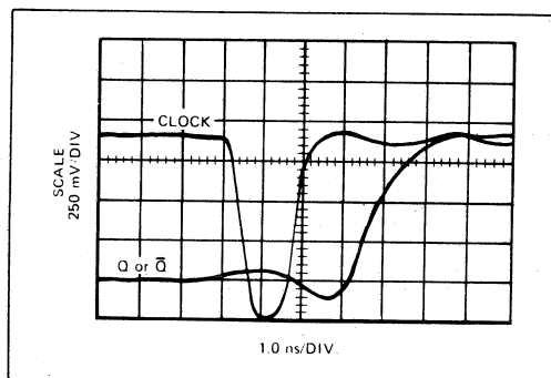
FIGURE 4 – MINIMUM “DOWN TIME” TO CLOCK OUTPUT LOAD = 50\Omega
