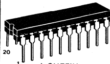
L SUFFIX CERAMIC PACKAGE CASE 732
