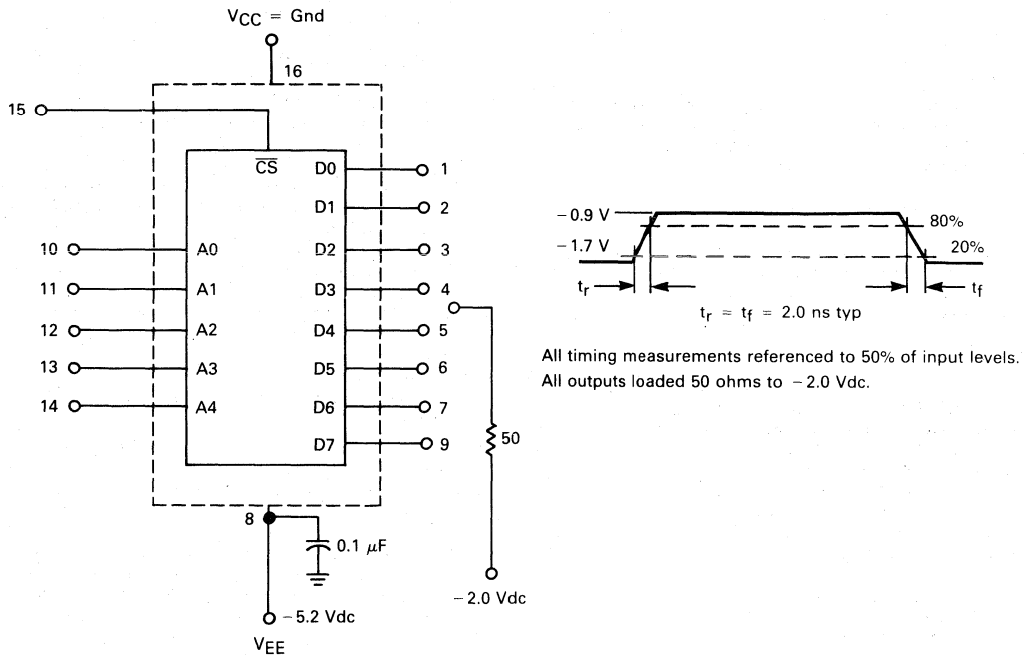
FIGURE 1 — SWITCHING TIME TEST CIRCUIT
