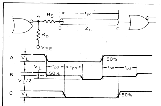
FIGURE 23 — SERIES TERMINATED LINE
