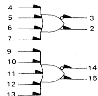
Dual 4-5 Input OR/NOR Gate
