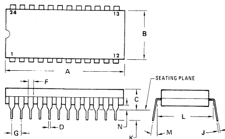
L SUFFIX CERAMIC PACKAGE CASE 623-05
