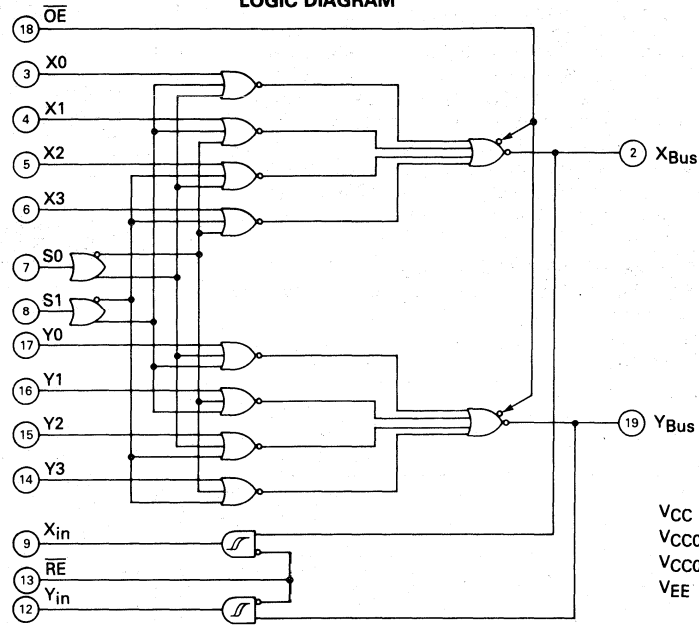
LOGIC DIAGRAM
