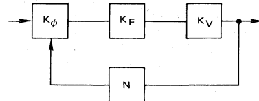
FIGURE 8 — GAIN CONSTANTS
