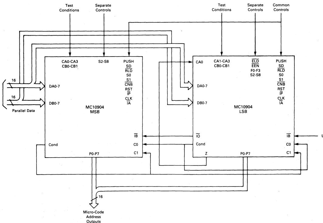
FIGURE 4 — 16 BIT MICRO-CODE SEQUENCER EXAMPLE
