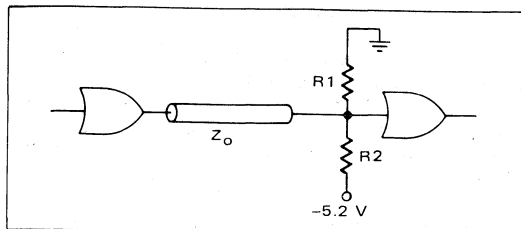
FIGURE 22b — PARALLEL TERMINATION—THEVENIN EQUIVALENT
