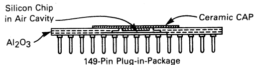
FIGURE 12 — CONSTRUCTION PROFILE
