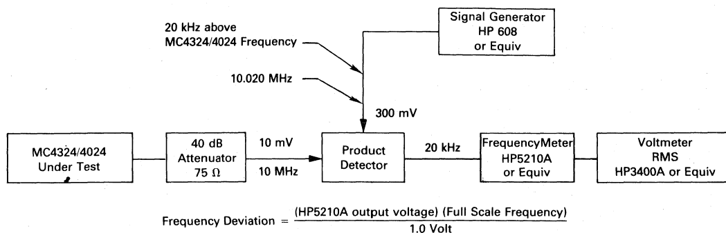
FIGURE 11 — NOISE DEVIATION TEST CIRCUIT
