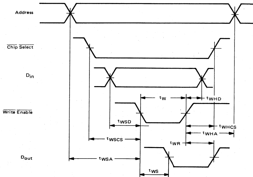
FIGURE 4 – WRITE MODE
