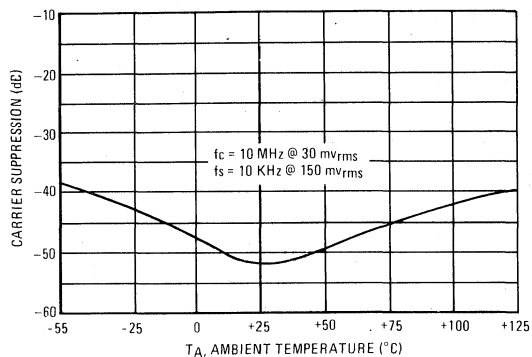
FIGURE 8 — CARRIER SUPPRESSION VERSUS TEMPERATURE
