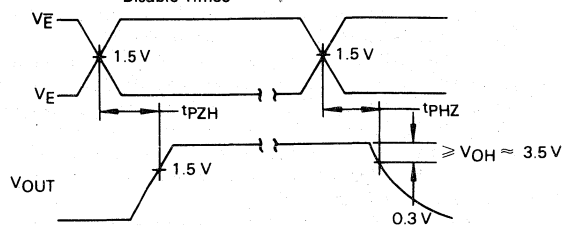
3-State Output High Enable and Disable Times
