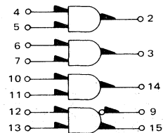
Quad 2-Input AND Gate
