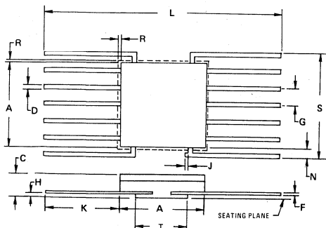
F SUFFIX CERAMIC PACKAGE CASE 607-04
