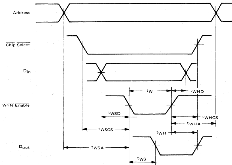
FIGURE 4 – WRITE MODE
