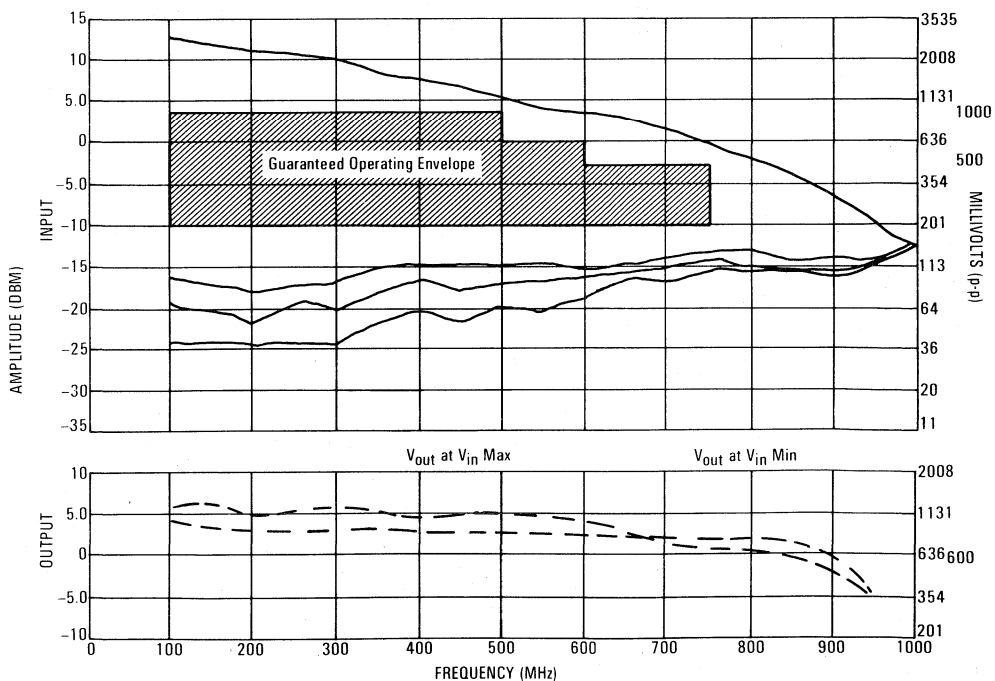
FIGURE 2 — GUARANTEED RANGE OF OPERATION (TEMP = 25°C, # DEVICES = FIVE; V_{CC} = 2.0\text{ V} , V_{EE} = -3.2\text{ V} , V_{BIAS} = 0.710\text{ V} )
