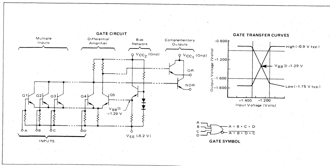
FIGURE 3 — MECL 10K GATE STRUCTURE AND SWITCHING BEHAVIOR
