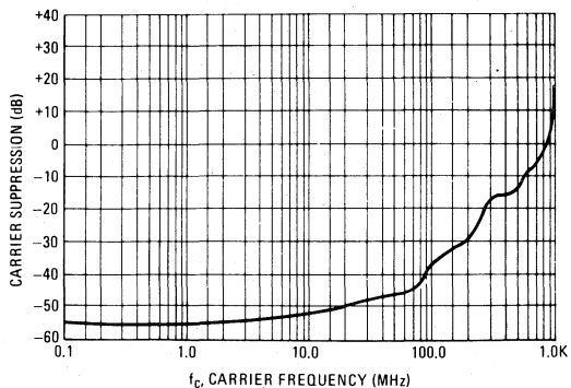
FIGURE 6 — CARRIER SUPPRESSION VERSUS FREQUENCY (Test 1)
