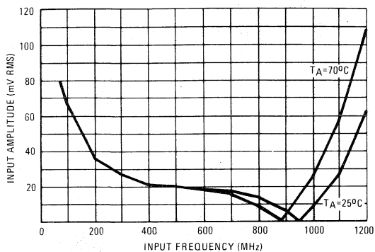
FIGURE 3 — TYPICAL UHF INPUT SENSITIVITY
