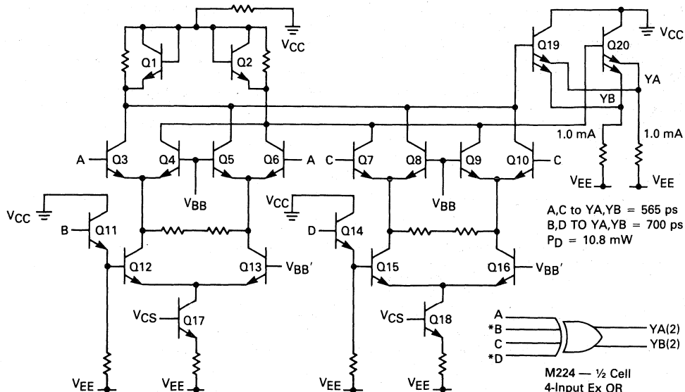
FIGURE 4 — SCHEMATIC OF 4-INPUT EXCLUSIVE OR GATE ( Y = ABCD + \bar{A}BCD + AB\bar{C}D + ABC\bar{D} + \bar{A}B\bar{C}D + \bar{A}BC\bar{D} + \bar{A}B\bar{C}\bar{D} + \bar{A}B\bar{C}\bar{D} )
