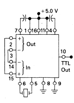
FIGURE 3 — MTTL OUTPUT
