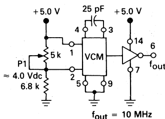
FIGURE 1 — ASTABLE MULTIVIBRATOR
