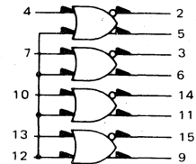
Quad OR/NOR Gate
