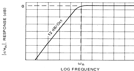
FIGURE 24 — LOOP RESPONSE TO VCO NOISE
