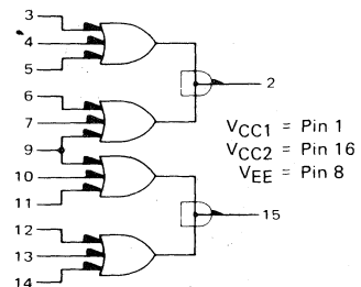
Dual 2-Wide 3-Input OR-AND Gate
