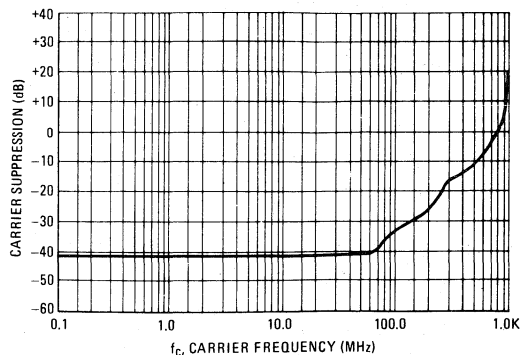
FIGURE 7 — CARRIER SUPPRESSION VERSUS FREQUENCY (Test 2)
