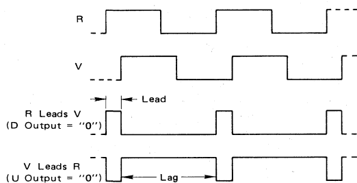
FIGURE 1 — TIMING DIAGRAM
