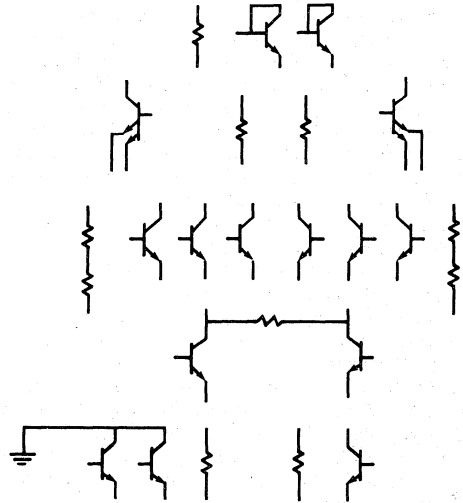
FIGURE 3 — OUTPUT CELL (O) SCHEMATIC
