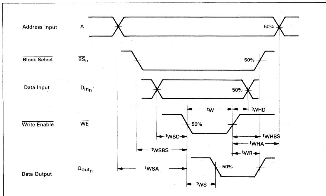
FIGURE 4 — WRITE STROBE MODE
