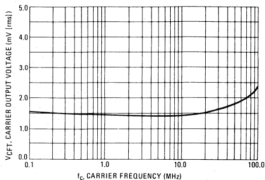
FIGURE 4 — CARRIER FEEDTHROUGH VERSUS FREQUENCY (Test 2)
