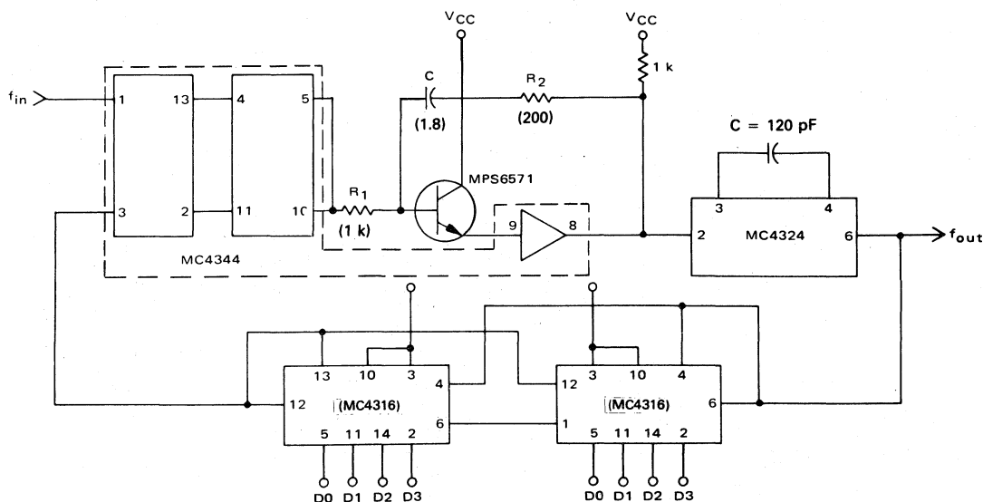
FIGURE 31 — CIRCUIT DIAGRAM OF TYPE 2 PHASE-LOCKED LOOP
