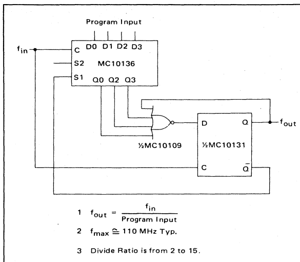
FIGURE 4 — 100 MHz PROGRAMMABLE COUNTER
