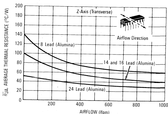
FIGURE 17A—AIRFLOW VERSUS THERMAL RESISTANCE (CERAMIC DUAL-IN-LINE PACKAGE)
