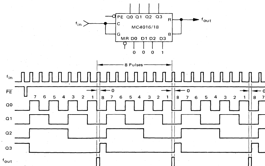
FIGURE 1 — SINGLE-STAGE OPERATION
