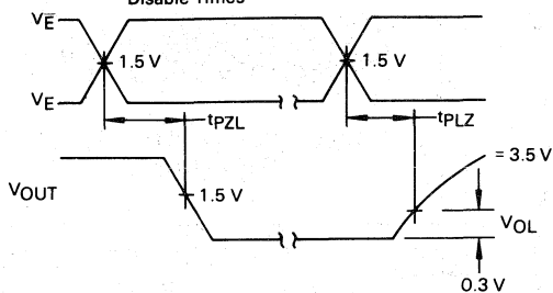
3-State Output Low Enable and Disable Times
