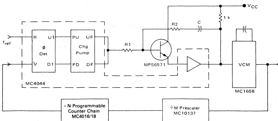
FIGURE 4 — TTL-MECL PHASE-LOCKED LOOP
