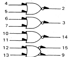
Quad 2-Input NOR Gate
