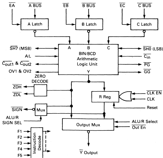
FIGURE 1 — 8-BIT BINARY/BCD ALU SLICE BLOCK DIAGRAM
