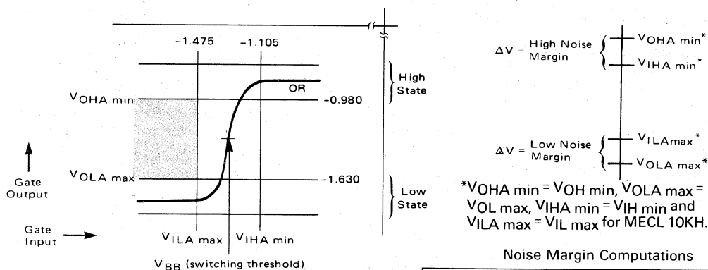
FIGURE 8 — MECL Noise Margin Data
