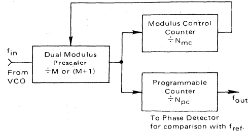
FIGURE 5 — FEEDBACK COUNTERS WITH DUAL MODULUS PRESCALER
