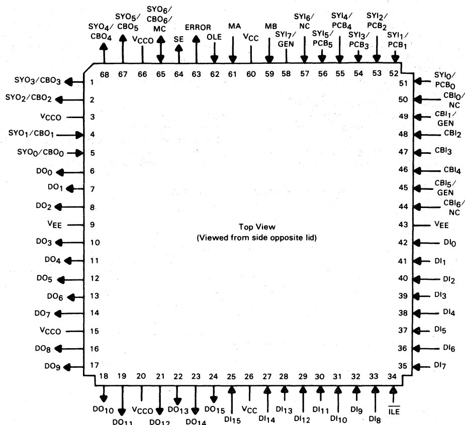
FIGURE 2 — INPUT/OUTPUT DIAGRAM
