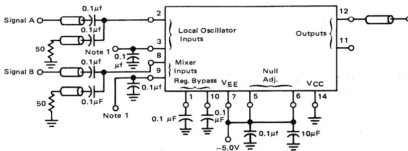
FIGURE 1 — A.C. GAIN TEST
