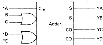
Logic Equivalent
