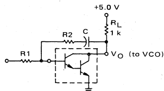
FIGURE 10 — USING MC4344/4044 LOOP AMPLIFIER
