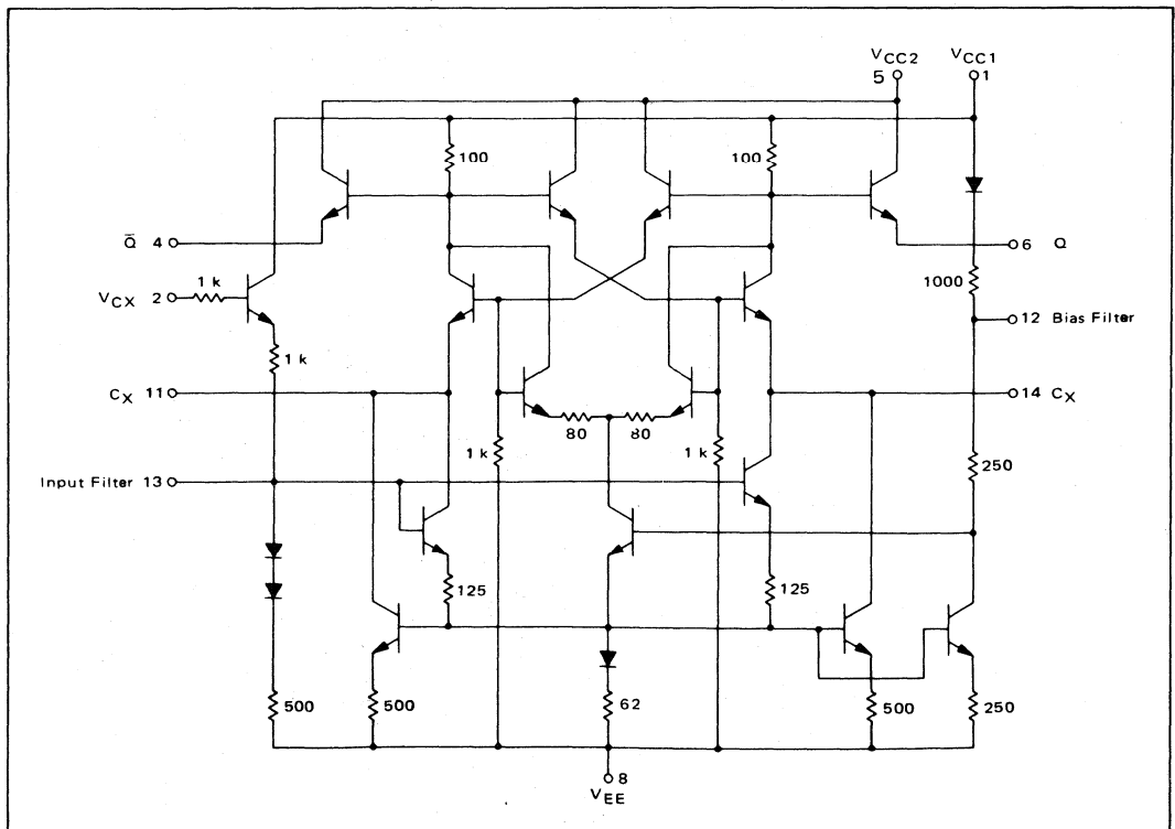
FIGURE 1 – CIRCUIT SCHEMATIC
