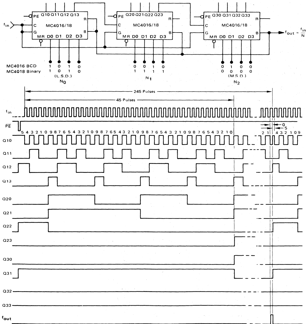
FIGURE 2 — CASCADED OPERATION
