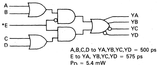
M254 — 2-to-1 Multiplexer w/Gated Inputs ¼ Cell
