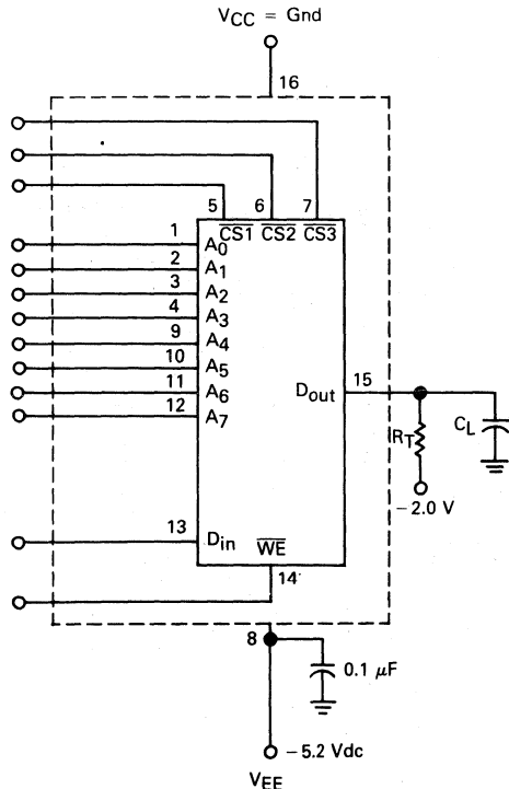
FIGURE 1 — SWITCHING TIME TEST CIRCUIT
