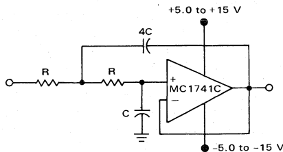
FIGURE 20 — OPERATIONAL AMPLIFIER LOW PASS FILTER
