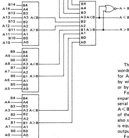
FIGURE 2 — 25-BIT MAGNITUDE COMPARATOR
