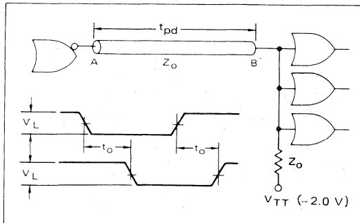
FIGURE 22a — PARALLEL TERMINATED LINE
