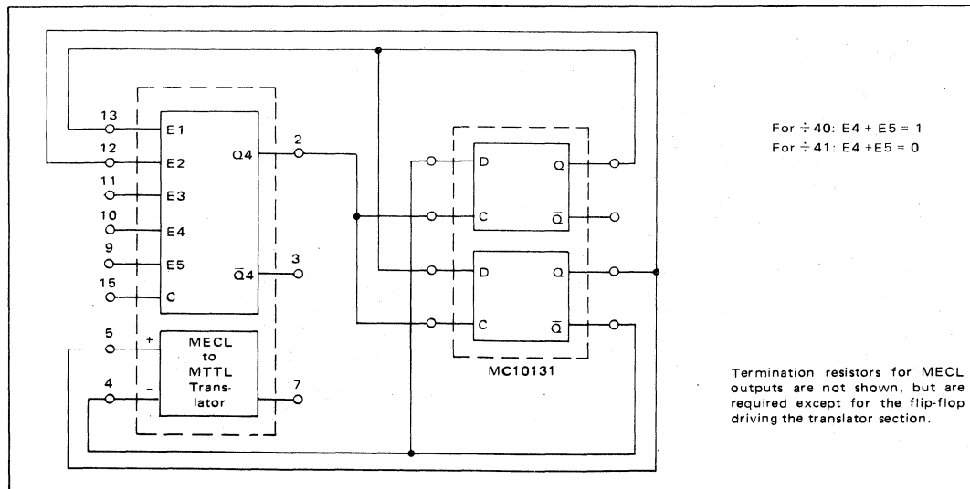
FIGURE 10 – DIVIDE BY 40/41 (MC12013/MC12513)
