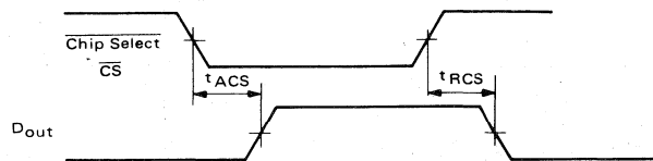
FIGURE 2 – CHIP SELECT ACCESS TIME
