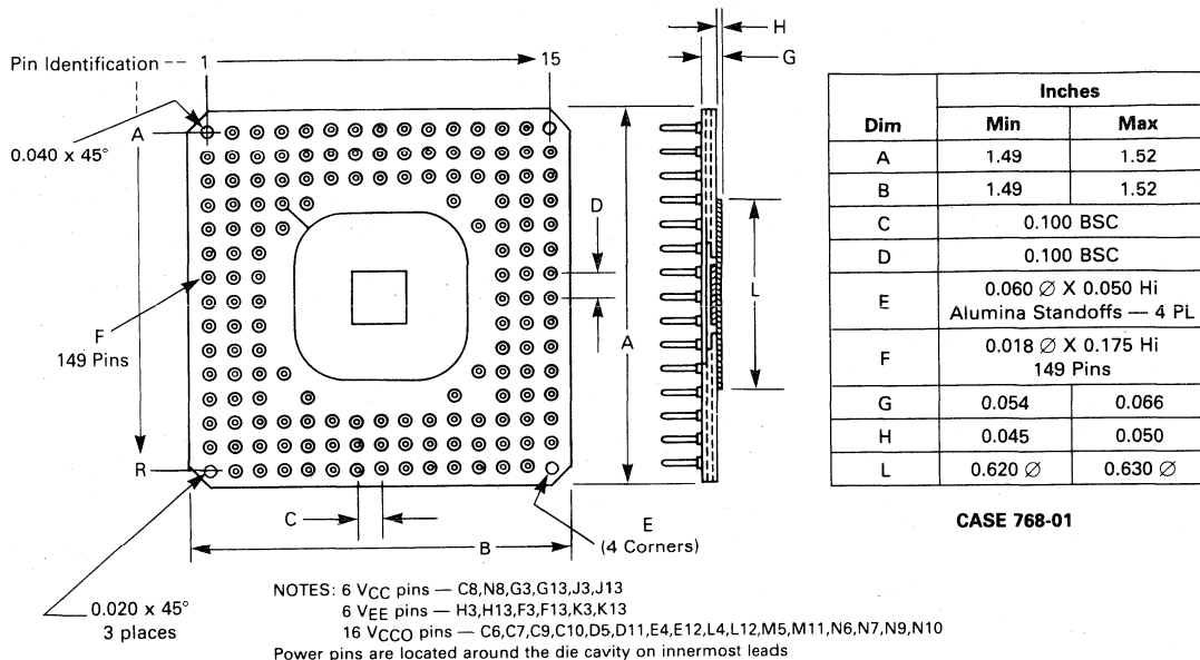
FIGURE 10 — PACKAGE DIMENSIONS
