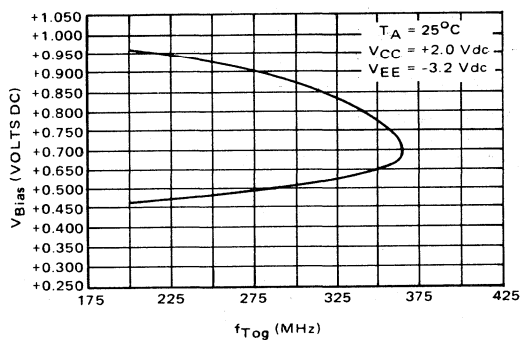
FIGURE 2 – MAXIMUM TOGGLE FREQUENCY (TYPICAL)
