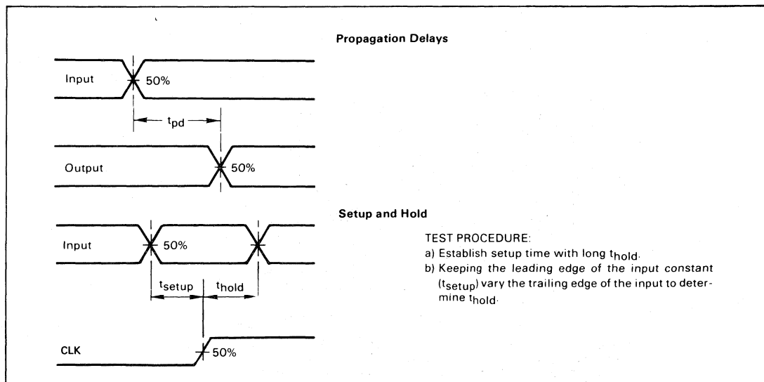
FIGURE 5 — SWITCHING WAVEFORMS
