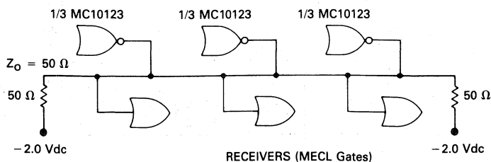
FIGURE 1 — 50-OHM BUS DRIVER
