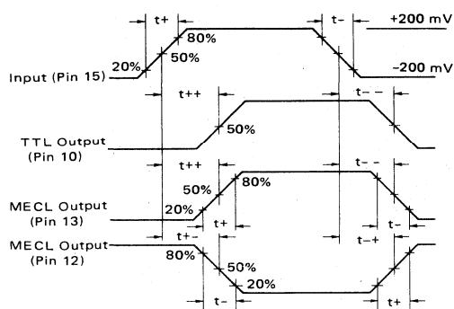
FIGURE 6 — AC CHARACTERISTICS — MECL AND TTL OUTPUTS
