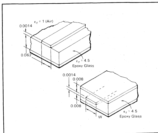
FIGURE 26 — PC INTERCONNECTION LINES FOR USE WITH MECL
