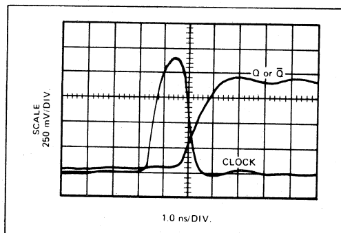
FIGURE 5 – MINIMUM “UP TIME” TO CLOCK OUTPUT LOAD = 50\Omega
