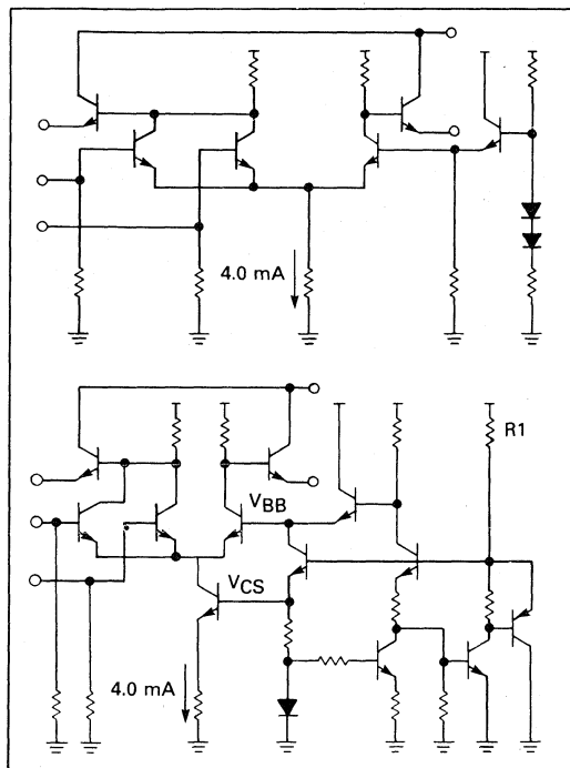
FIGURE 1 — MECL 10K versus MECL 10KH GATE DESIGN
