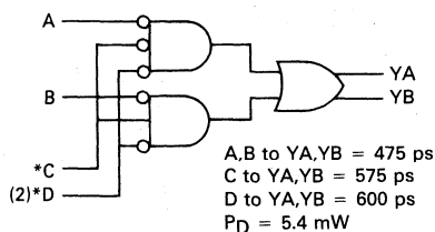
M253 — 2-to-1 Multiplexer w/Enable ¼ Cell
