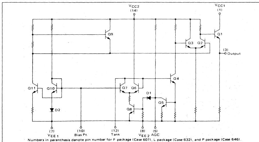
FIGURE 1 — CIRCUIT SCHEMATIC
