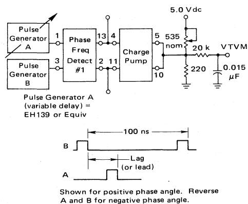
FIGURE 5 — PHASE DETECTOR TEST
