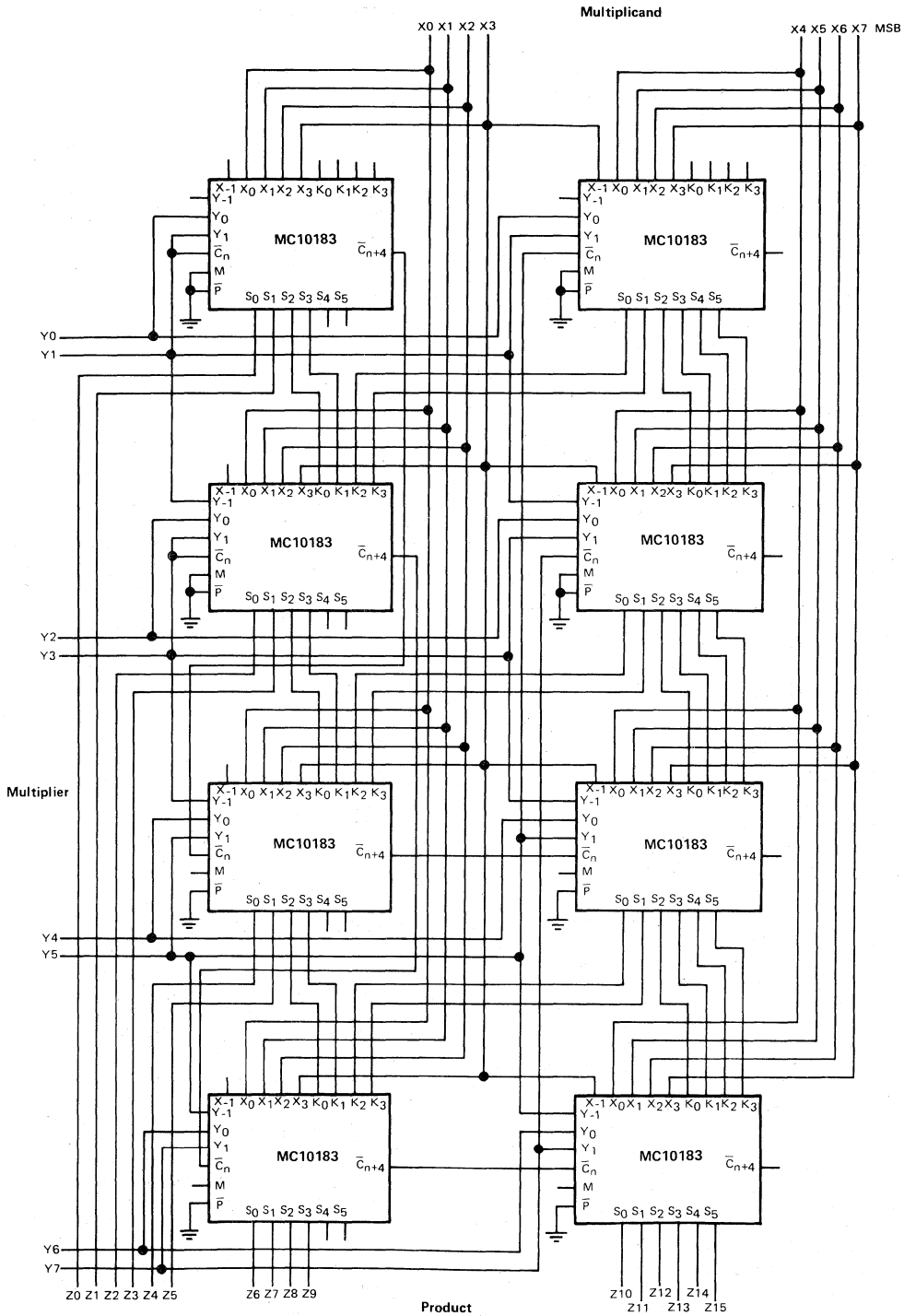
FIGURE 1 – 8-BIT X 8-BIT 2's COMPLEMENT MULTIPLIER
