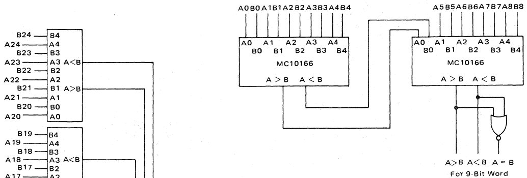
FIGURE 1 — 9-BIT MAGNITUDE COMPARATOR
