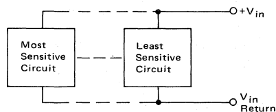
FIGURE 27 — REGULATOR GROUND CONNECTION
