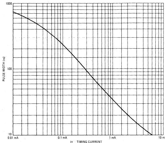
FIGURE 5 — PULSE WIDTH versus I_T @ C_{Ext} = 13 pF
