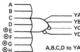
M203 — 8-Input OR/NOR ½ Cell
