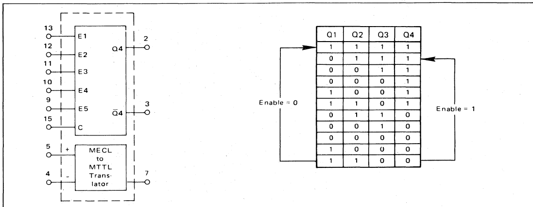
FIGURE 8 — DIVIDE BY 10/11 (MC12013/MC12513)
