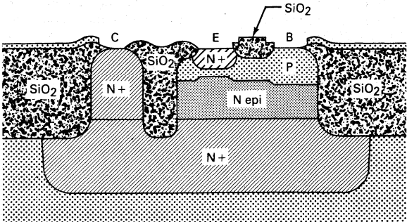
FIGURE 5 — CROSS SECTION of MOSAIC II PROCESS
