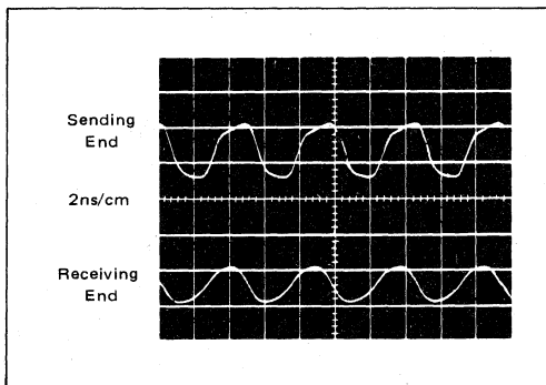
FIGURE 2 – 400 MBS WAVEFORMS
