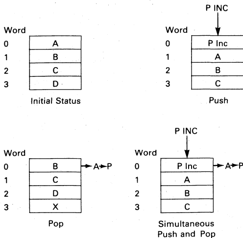
FIGURE 3 — MC10904 Stack Operation
