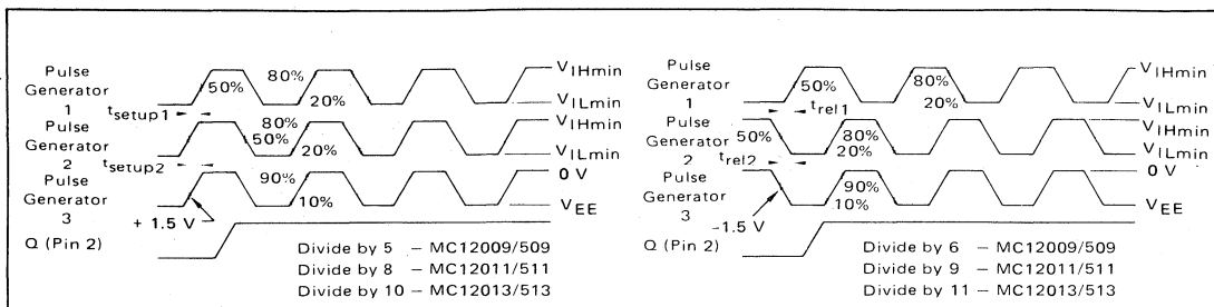
FIGURE 4 – SETUP AND RELEASE TIME WAVEFORMS
