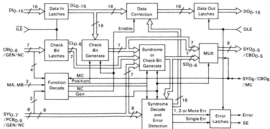
BLOCK DIAGRAM — FIGURE 1
