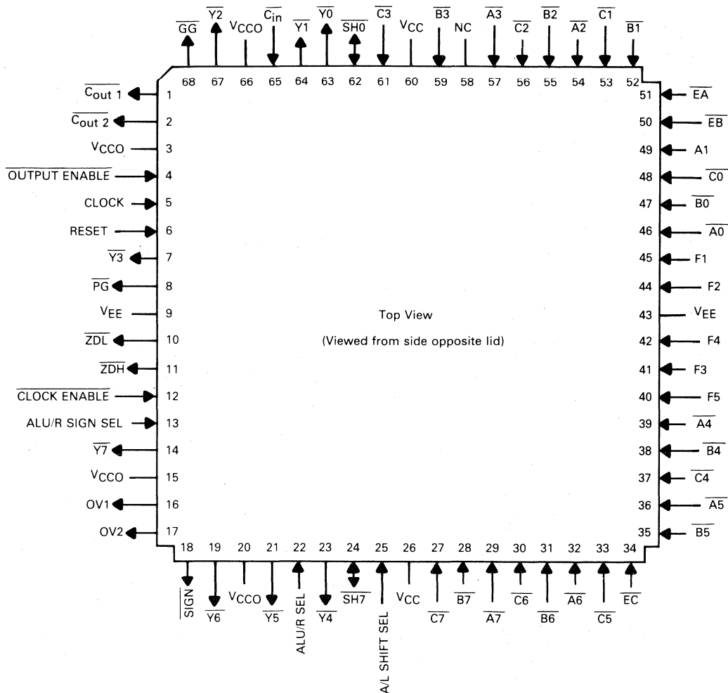
FIGURE 2 — INPUT/OUTPUT DIAGRAM
