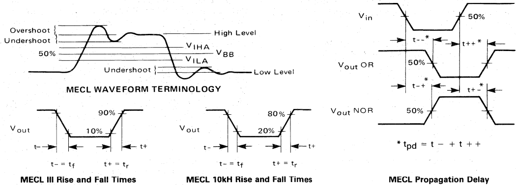
FIGURE 9 — TYPICAL LOGIC WAVEFORMS
