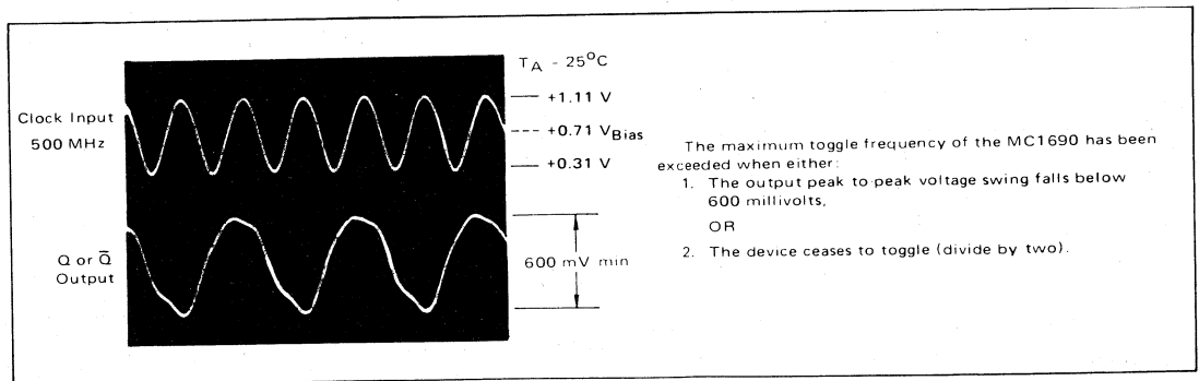
FIGURE 2 – TOGGLE FREQUENCY WAVEFORMS
