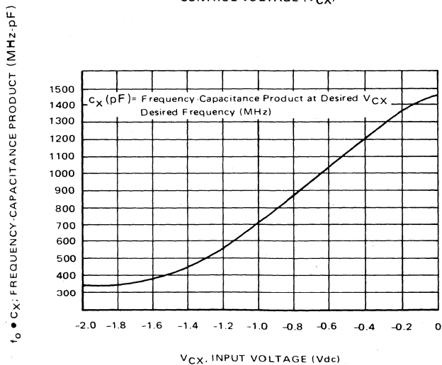
FIGURE 5 — FREQUENCY-CAPACITANCE PRODUCT versus CONTROL VOLTAGE ( V_{CX} )
