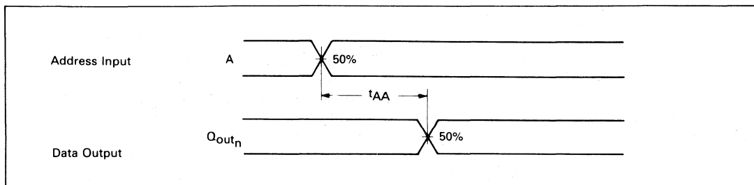
FIGURE 3 — ADDRESS ACCESS TIME
