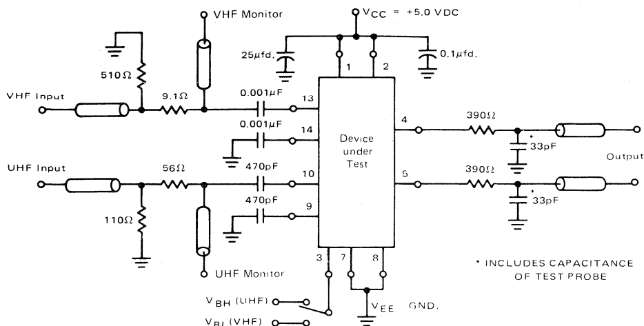
STANDARD TEST FIXTURE
