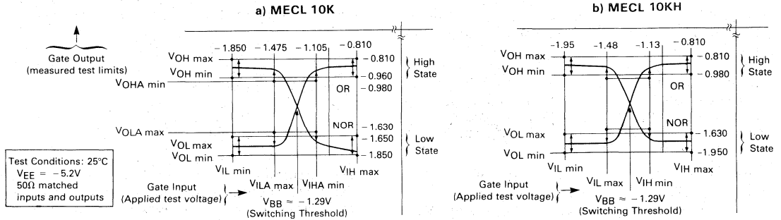
FIGURE 5 — MECL TRANSFER CURVES and SPECIFICATION TEST POINTS
