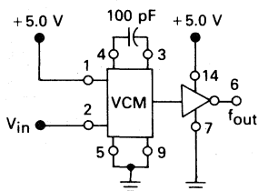
FIGURE 3 — VOLTAGE-CONTROLLED MULTIVIBRATOR
