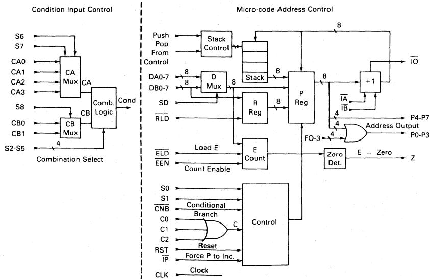
FIGURE 1 — 8-BIT MICRO-CODE SEQUENCER BLOCK DIAGRAM
