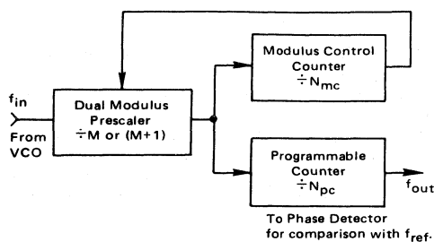
FIGURE 6 — FEEDBACK COUNTERS WITH DUAL MODULUS PRESCALER
