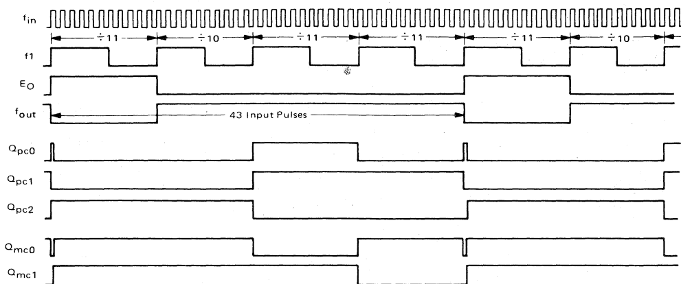
FIGURE 7a — DIVISION BY 43
