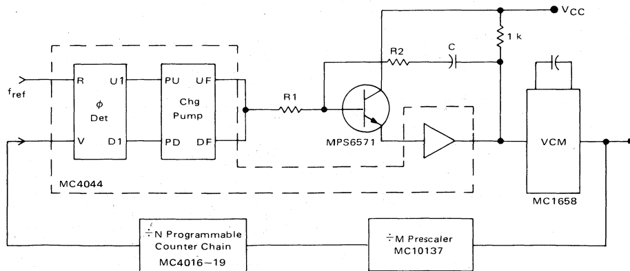
FIGURE 5 — MTTL-MECL PHASE-LOCKED LOOP
