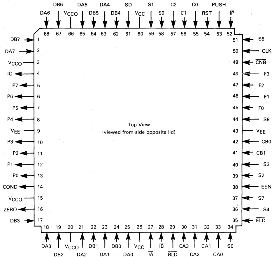
FIGURE 2 — INPUT/OUTPUT DIAGRAM
