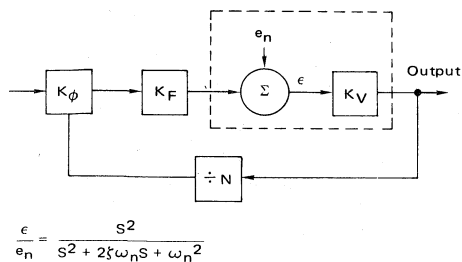
FIGURE 23 — EFFECTS OF VCO NOISE
