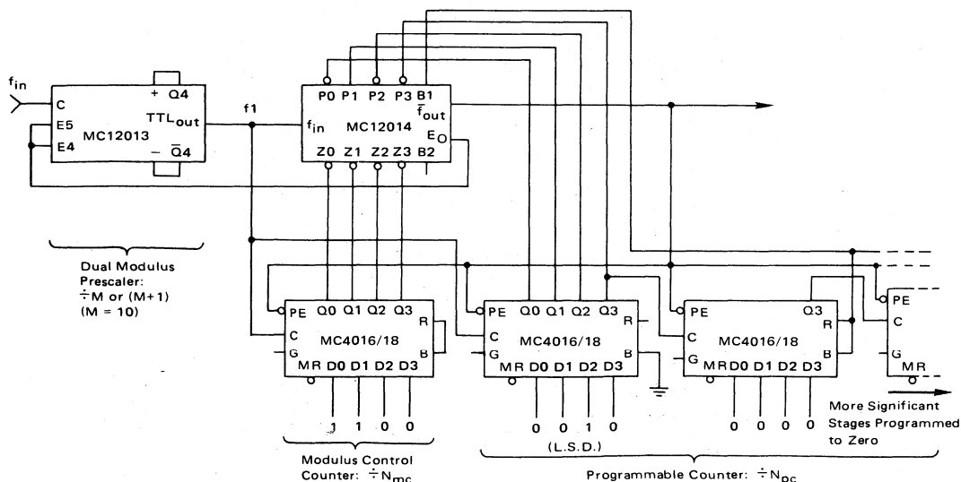
FIGURE 7 — FREQUENCY DIVISION: f_O = f_{in}/MN_{pc} + N_{mc}
