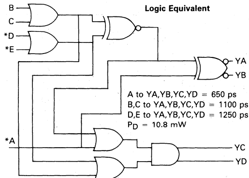
Logic Equivalent
