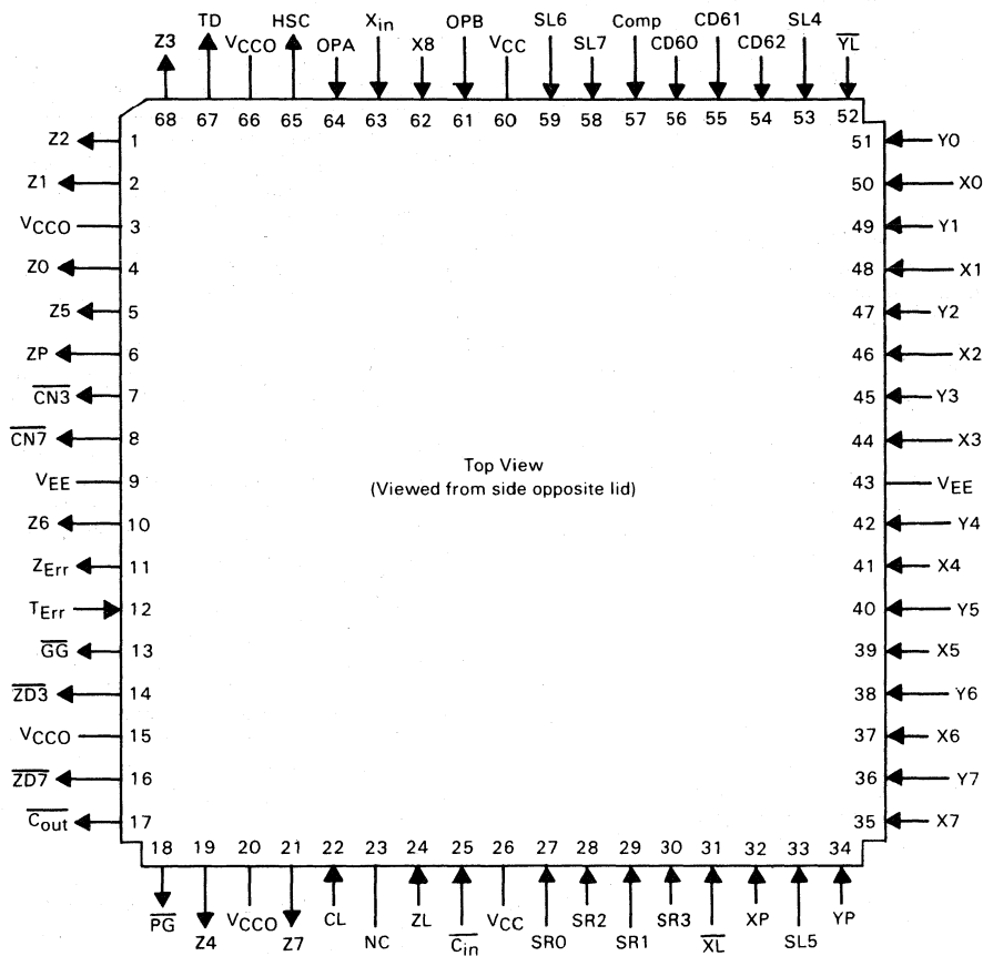
FIGURE 2 — INPUT/OUTPUT DIAGRAM
