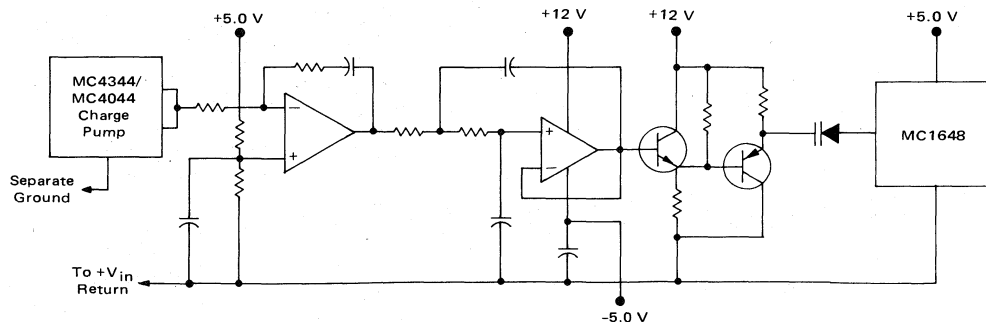
FIGURE 28 — PARTIAL SCHEMATIC OF LOOP AMPLIFIER AND FILTER
