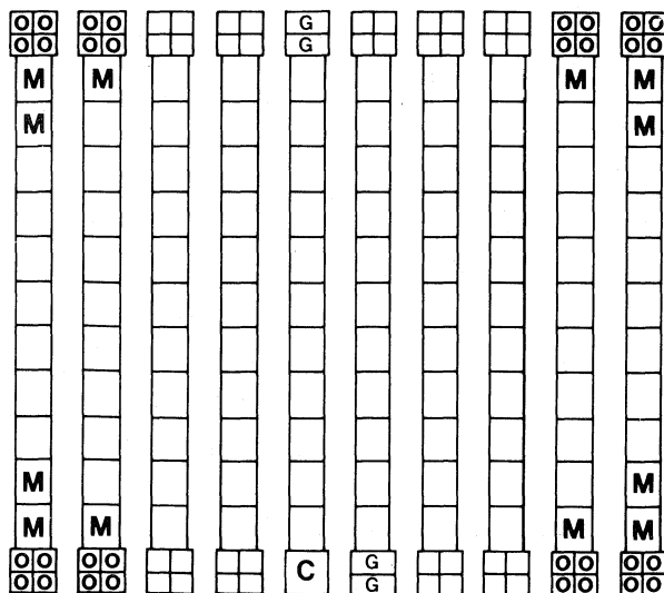
FIGURE 1 — MCA2500ECL MACROCELL ARRAY LAYOUT
