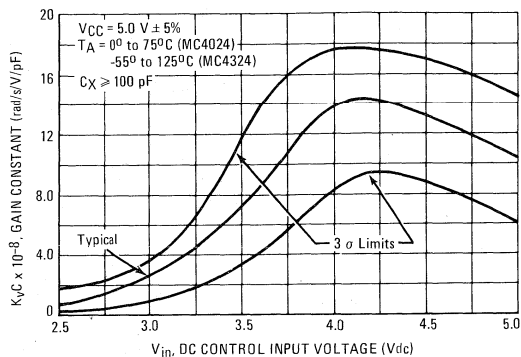
FIGURE 6 — FREQUENCY-VOLTAGE GAIN CHARACTERISTICS
