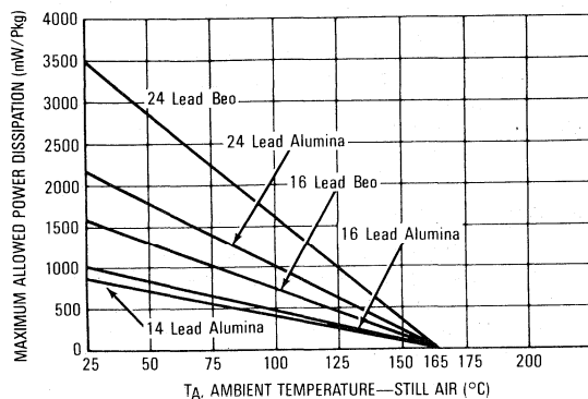
FIGURE 16B—AMBIENT TEMPERATURE DERATING CURVES (CERAMIC FLAT PACKAGE)
