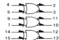
Triple 2-Input Exclusive OR/NOR Gate
