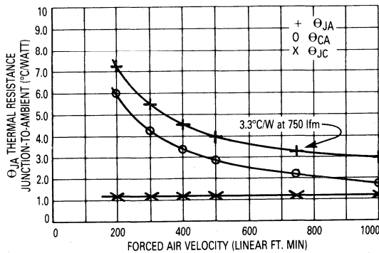
FIGURE 11 — THERMAL CHARACTERISTICS (TYPICAL)
