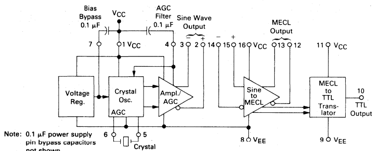
TYPICAL CIRCUIT CONFIGURATIONS Note: 0.1 \mu F power supply pin bypass capacitors not shown.
