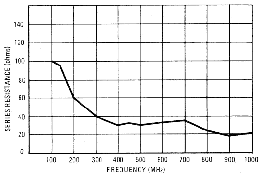
FIGURE 5 — TYPICAL INPUT IMPEDANCE
