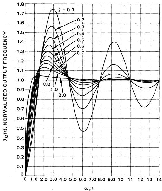
FIGURE 9 — TYPE 2 SECOND ORDER STEP RESPONSE
