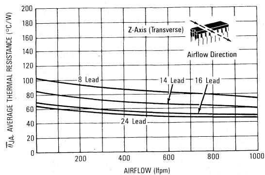
FIGURE 17C—AIRFLOW VERSUS THERMAL RESISTANCE (PLASTIC DUAL-IN-LINE PACKAGE)
