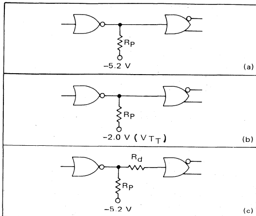
FIGURE 21 — PULL-DOWN RESISTOR TECHNIQUES
