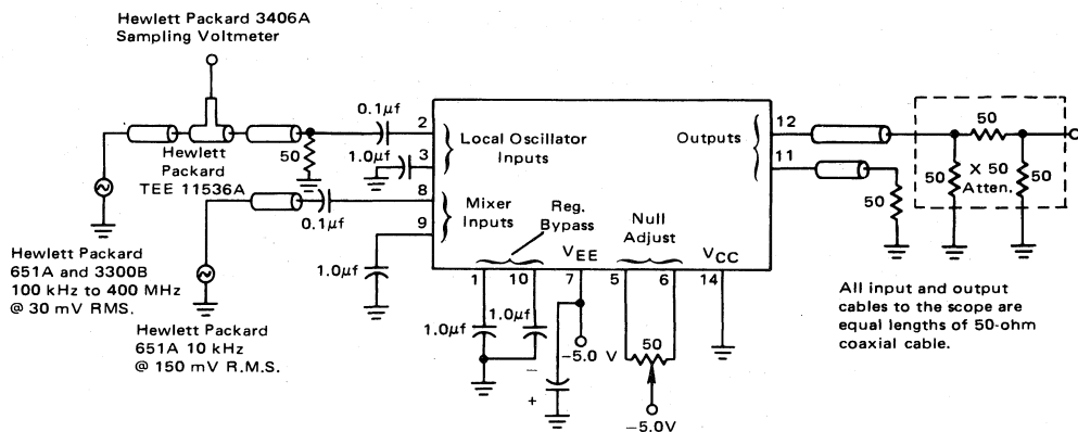
FIGURE 5 — CARRIER SUPPRESSION TEST CIRCUIT
