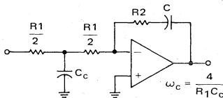
FIGURE 16 — IMPROVED TRANSIENT SUPPRESSION WITH R2 - C_c
