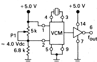
FIGURE 2 — CRYSTAL CONTROLLED MULTIVIBRATOR
