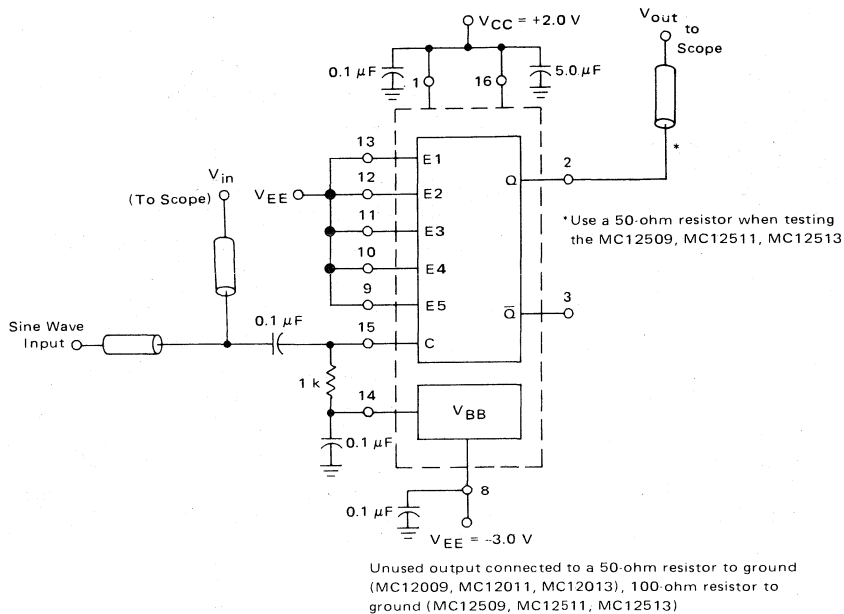
FIGURE 6 – MAXIMUM FREQUENCY TEST CIRCUIT
