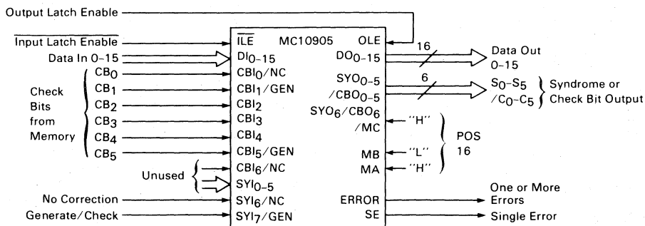
FIGURE 3 — 16-BIT DATA CONFIGURATION
