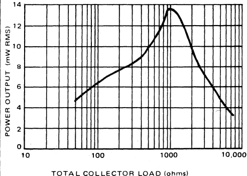
See test circuit, Figure 12, f = 10 \text{ MHz} C3 = 470 \text{ pF} Collector Tank L1 = 2.7 \mu\text{H} C1 = 24 \dots 200 \text{ pF} R = 50 \Omega - 10 \text{ k}\Omega R_p \text{ of } L1 \text{ and } C1 = 6.8 \text{ k}\Omega @ 10 \text{ MHz Resonance} Oscillator Tank L2 = 2.7 \mu\text{H} C2 = 16 - 150 \text{ pF}
