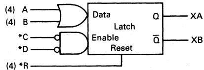
X292 — Gated Latch One Cell
