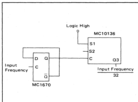
FIGURE 2 — 300 MHz PRESCALER
