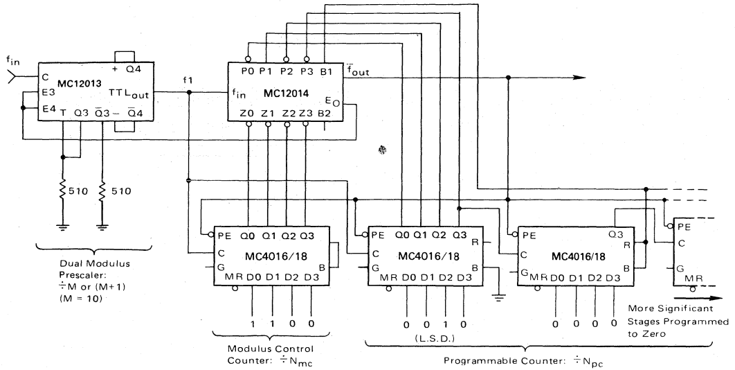
FIGURE 6 — FREQUENCY DIVISION: f_0 = f_{in}/(MN_{pc} + N_{mc})
